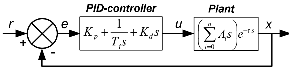
Figure 1. Scheme of the closed-loop controlled plant
